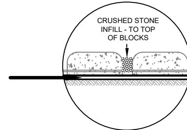
OPTIONAL STONE INFILL, USE 10 OZ. NON-WOVEN GEOTEXTILE UNDERLAYMENT
