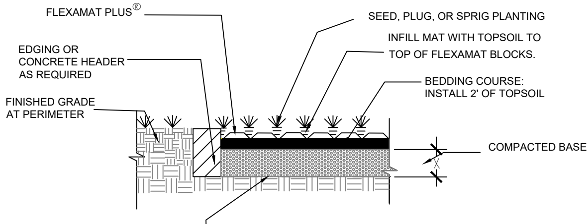
OPTIONAL STONE INFILL, USE 10 OZ. NON-WOVEN GEOTEXTILE UNDERLAYMENT
