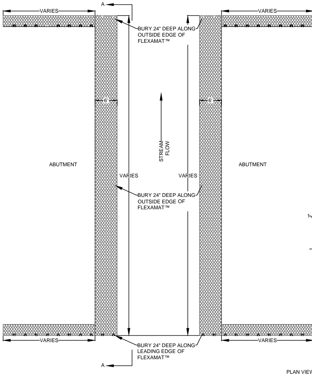
PLAN VIEW
